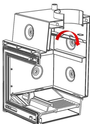
Figure No.21 - Dismantling the upper Sarria Plus deflector
