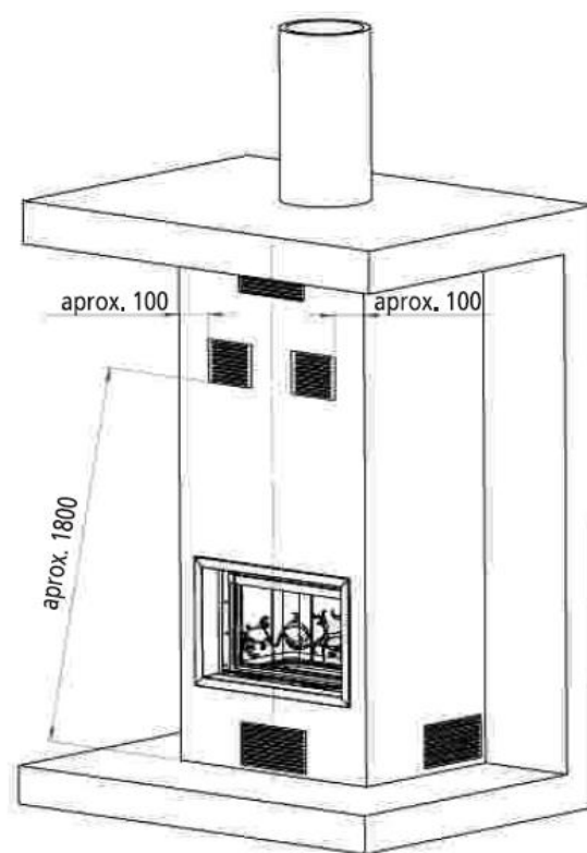
Figure No.8 - Exterior diagram of the casing
