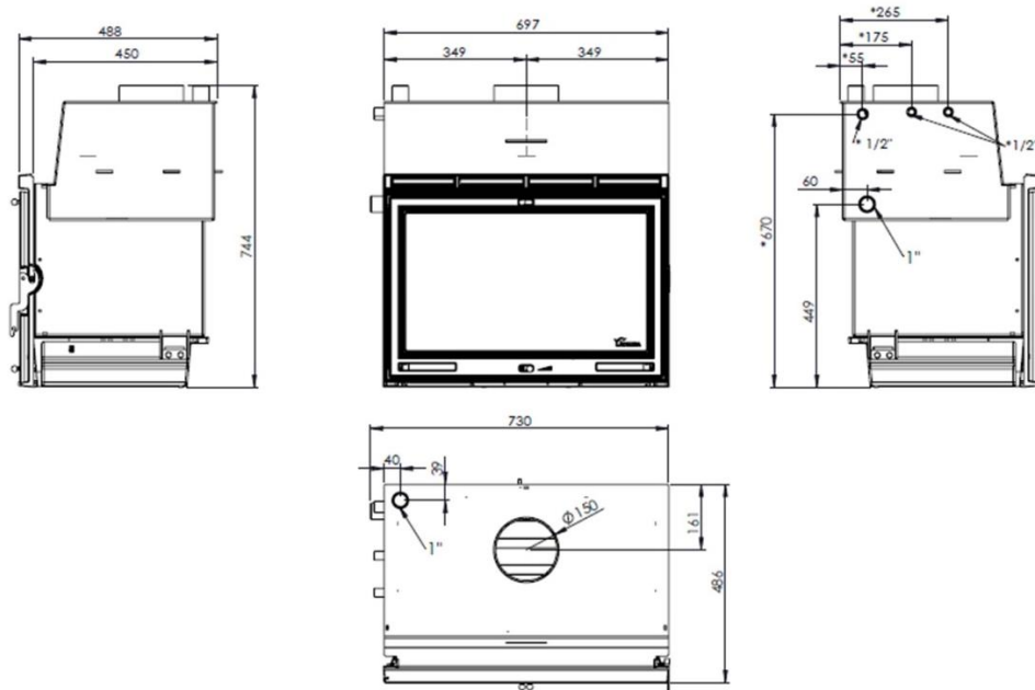
Figure No.2 - Dimensions of the SARRIA SAKAN 9 appliance in mm
