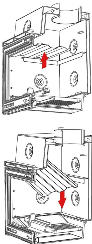
Figure No.18 - Dismantling the Sarria deflector
