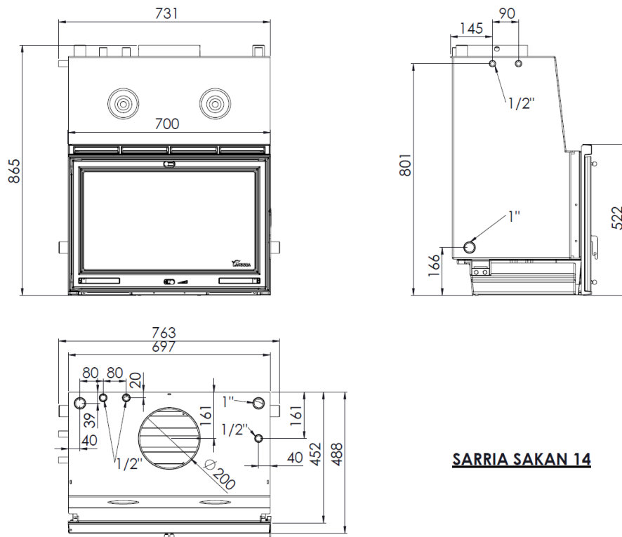
Figure No.4 - Dimensions of the SARRIA SAKAN 14 appliance in mm
