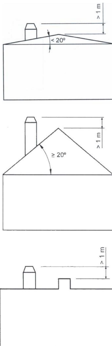
Figure No.12 - Distances between chimney crown and roof ridge
