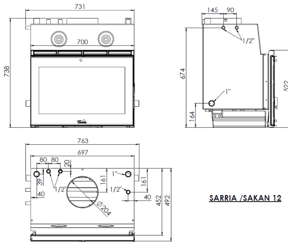
Figure No.3 - Dimensions of the SARRIA SAKAN 12 appliance in mm
