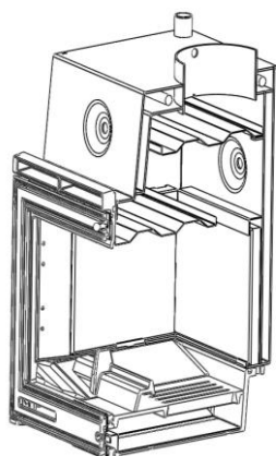
Figure No.22 - Section view with two deflectors fitted (Sarria Plus)
