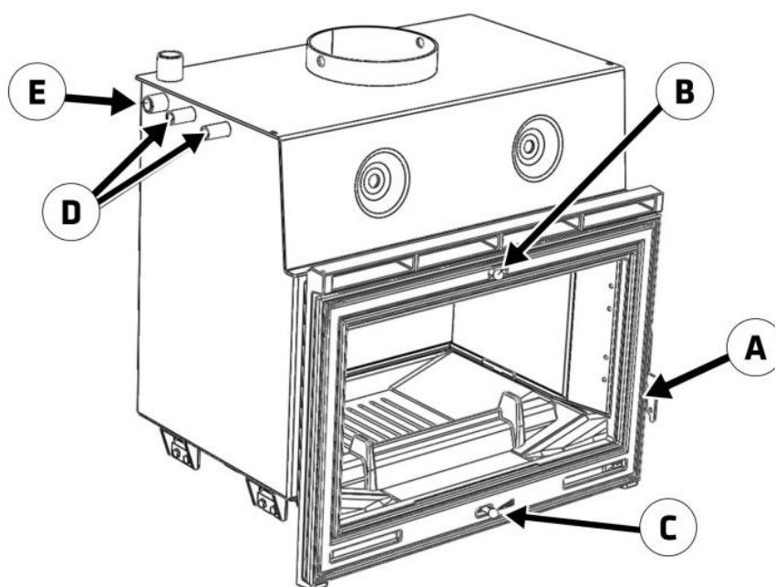
Figure No.17 - Operating components on the appliance
