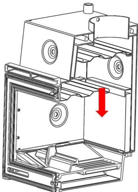
Figure No.9 - Insert the part at an angle and pushing upwards in order to clear the strip at the bottom and let it drop
