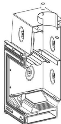
Figure No.19 - Section view with one deflector fitted (Sarria)
