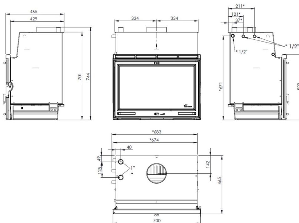
Figure No.1 - Dimensions of the SARRIA SAKAN 6 appliance in mm
