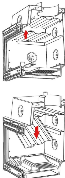
Figure No.20 - Dismantling the lower Sarria Plus deflector
