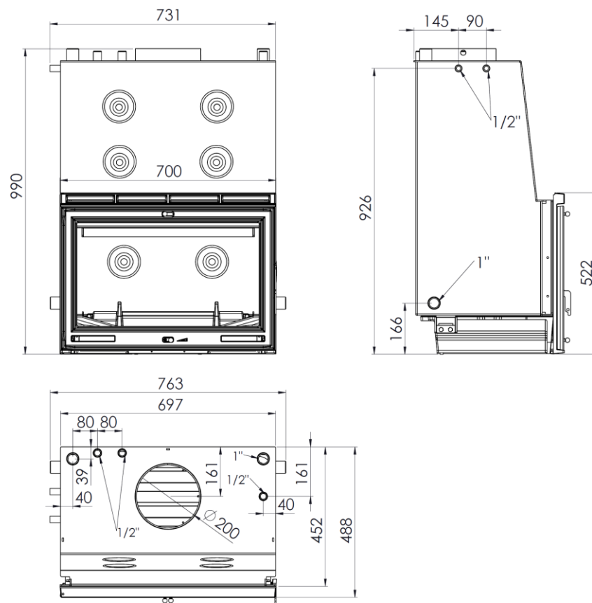
Figure No.5 - Dimensions of the SARRIA SAKAN 16 appliance in mm
