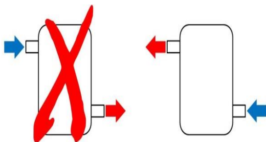
Figure No.15 - Wrong connection (left) and Right connection (right)
