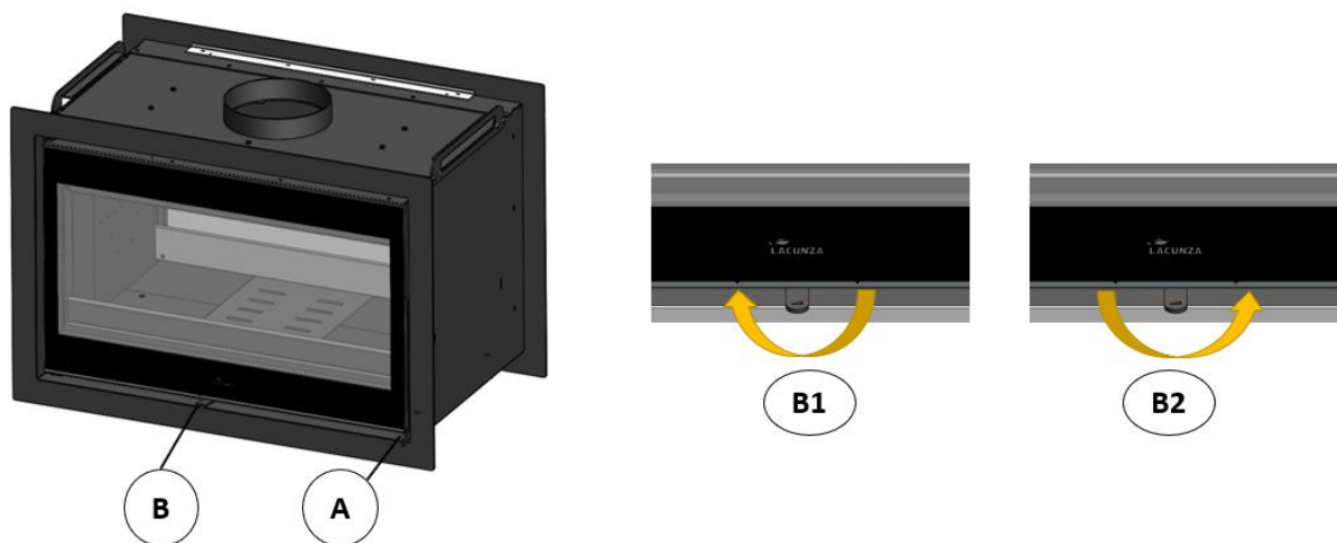
Figure No.16 - Operating components on the appliance
