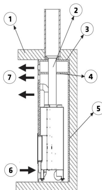
Figure No.4 - Interior diagram of the casing
