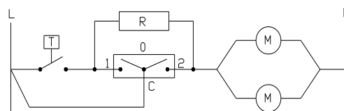
Figure No.11 - Electrical diagram for fans
