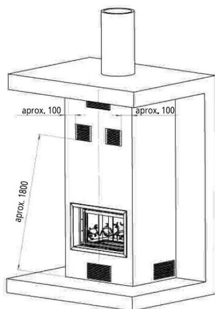
Figure No.5 - Exterior diagram of the casing
