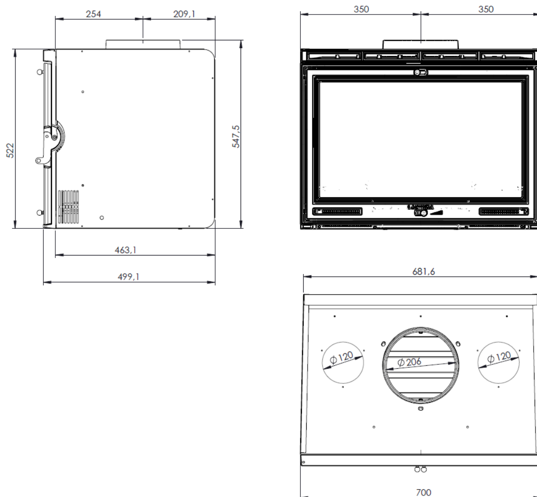
Figure No.1 - Dimensions of the IN- 700 appliance in mm
