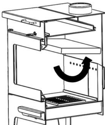
Figure No.11 - Turn the deflector upwards at the rear and leave it horizontally raised
