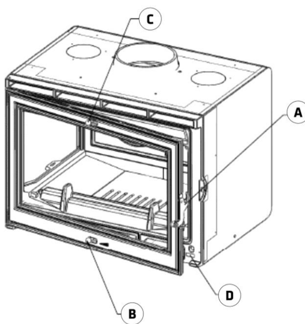
Figure No.10 - Operating components on the appliance
