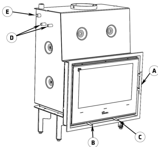
Figure No.14 - Operating components on the appliance
