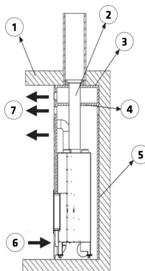
Figure No.3 - Interior diagram of the casing
