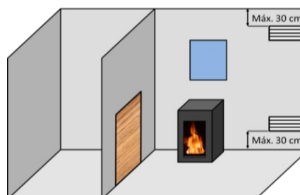
Figure No.2 - Guideline indications for ventilation grilles
