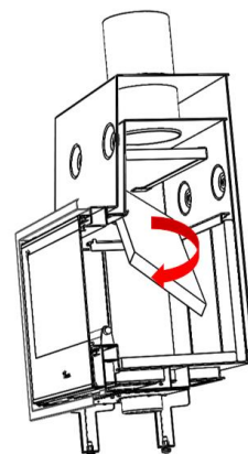
Figure No.15 - Dismantling the lower Otazu Plus deflector
