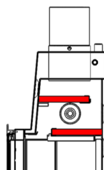
Figure No.17 - Section view with two deflectors fitted Otazu Plus.
