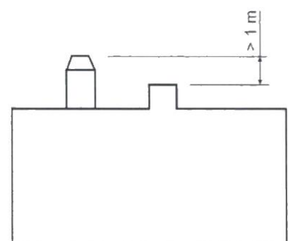
Figure No.7 - Distances between chimney crown and roof ridge
