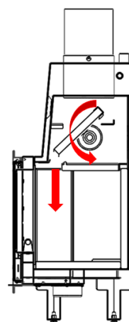
Figure No.16 - Dismantling the upper Otazu Plus deflector
