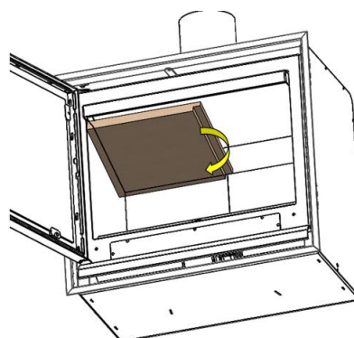
Figure No.17 - Extracting the vermiculite deflectors
