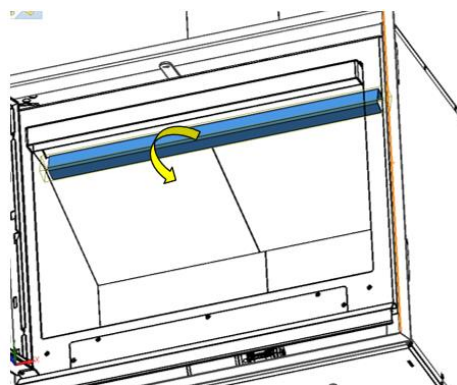
Figure No.16 - First movement to release the reinforcement
