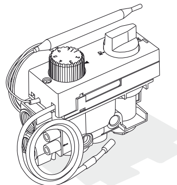
Battery operated remote ignition and control (GV60)
