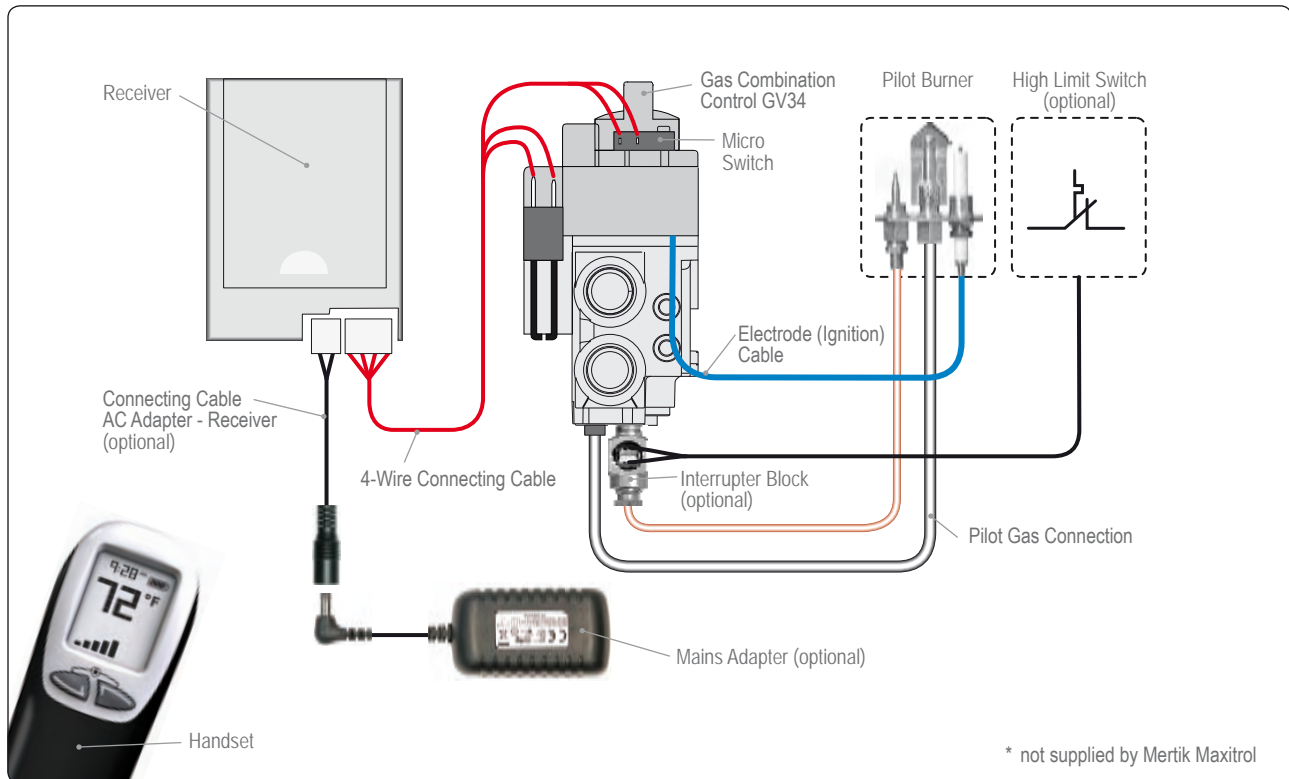
Illustration 12: GV34 - Electronic Options
