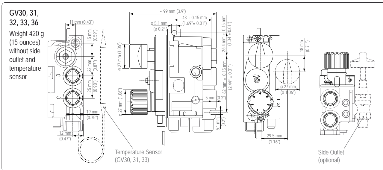
Illustration 5: GV30, 31, 32, 33, 36 - Dimensions and Weight
