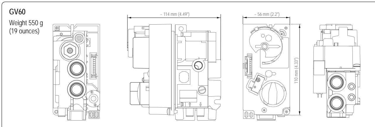
Illustration 7: GV60 Series - Dimensions and Weight
