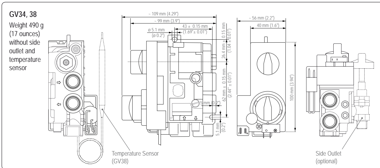
Illustration 6: GV34, 38 - Dimensions and Weight
